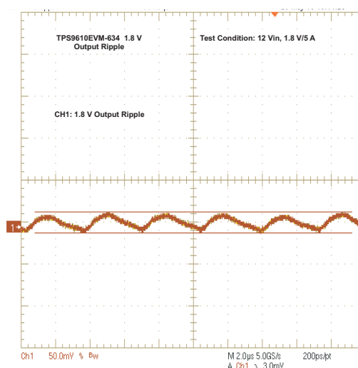
Figure 53. 1.8-V V_O Ripple
