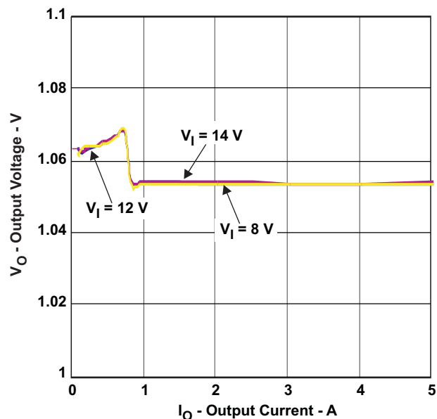
Figure 55. 1.05-V Load Regulation
