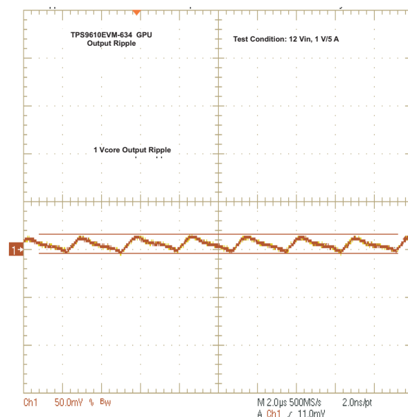
Figure 26. GPU Vcore Ripple
